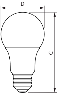
Bulb A19 120V 8.8-60W 800lm 2700K E26 D
