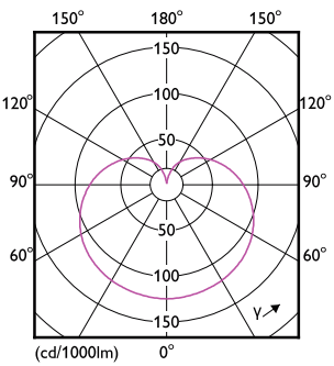
LED Bulb A19 E26 5-40W
