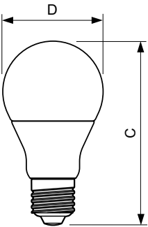
Bulb A19 5-40W 450lm 2200-2700K E26 D
