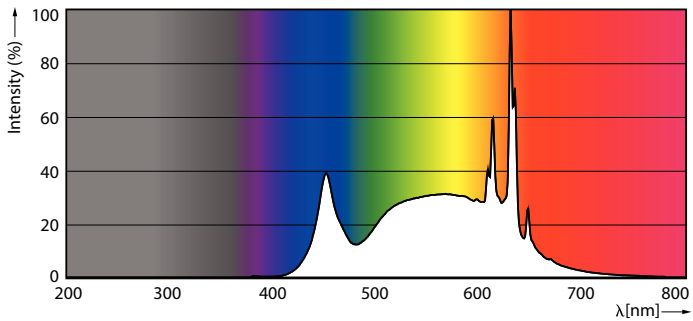
Spectral Power Distribution Colour - 12.2A19/PER/940/P/E26/DIM 6/1FB T20
