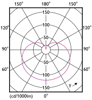
Light Distribution Diagram - 12.2A19/PER/940/P/E26/DIM 6/1FB T20
